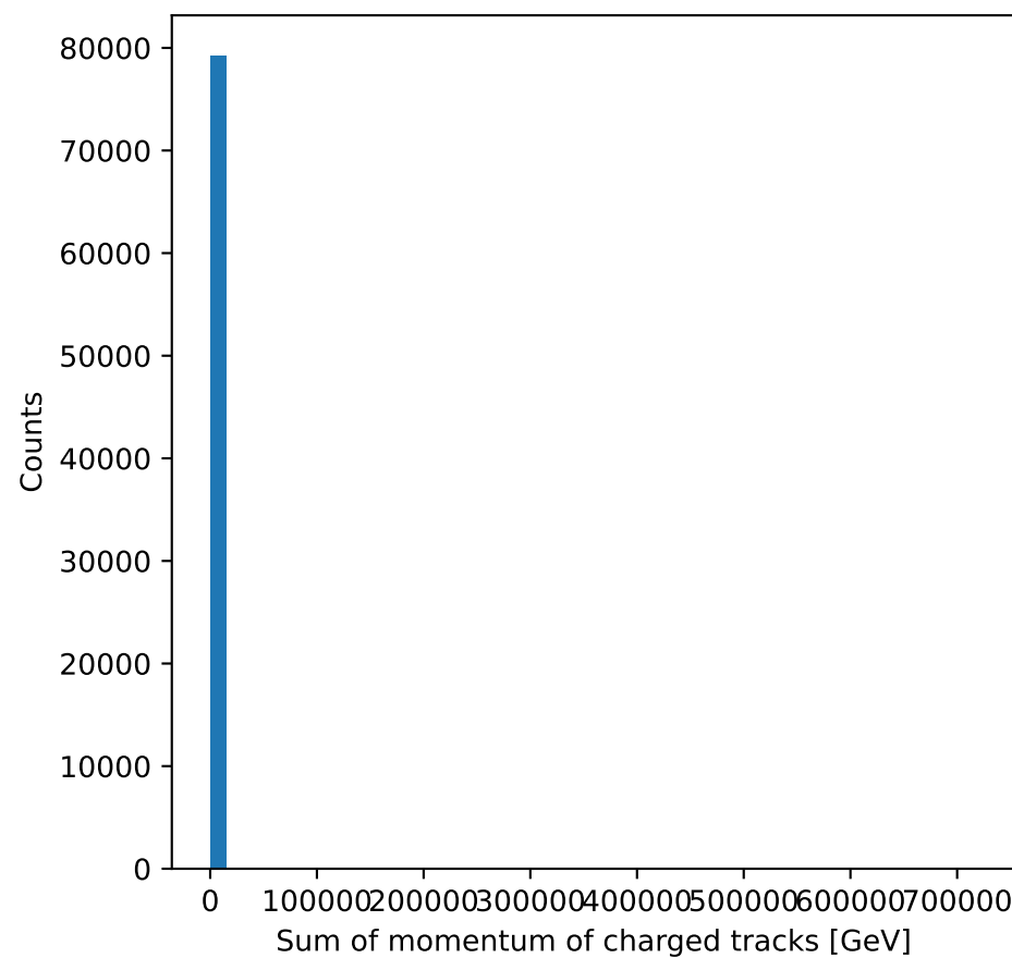
\tau^+\tau^- channel
